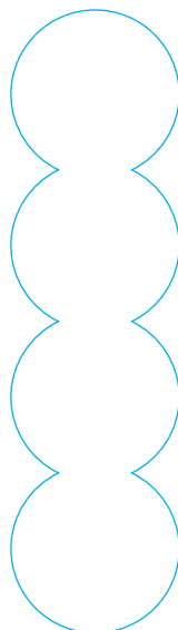
74mm x 20mm 4up flexible die Die code: M74x20v4 Order Code: V7
